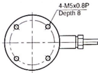
Bottom View (50 - 1000kg)
