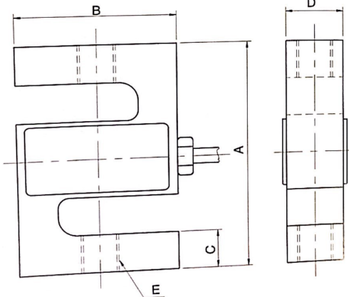
Dimension-mm(inch)
